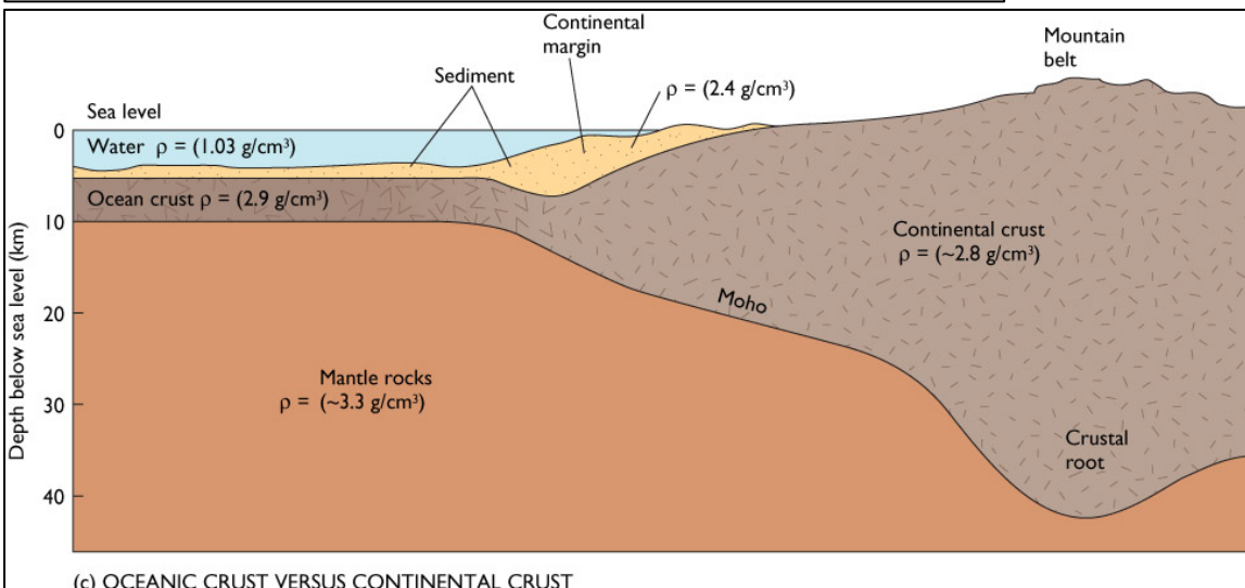
(c) OCEANIC CRUST VERSUS CONTINENTAL CRUST
