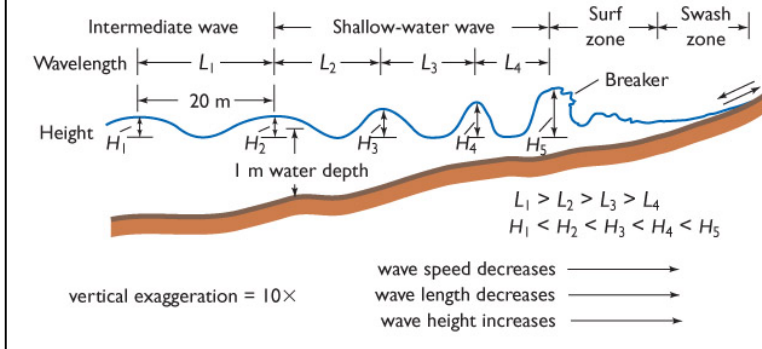
(b) SHALLOW-WATER WAVES IN PROFILE
