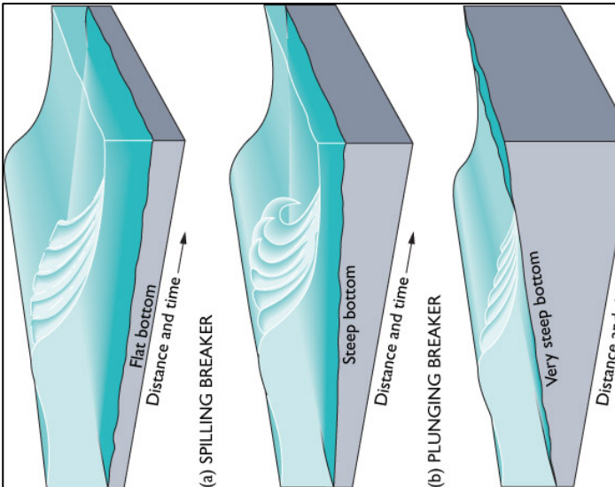
(a) SPILLING BREAKER
