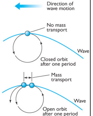
(c) STOKES DRIFT
