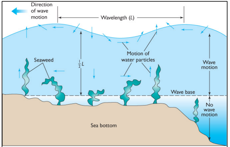
(a) WAVE MOTION WITH DEPTH
