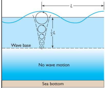
(b) ORBITS OF WATER PARTICLES
